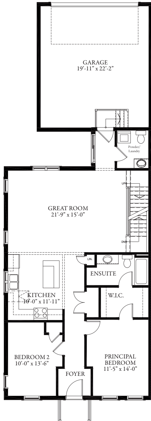
END UNIT | GROUND FLOOR 1247 Square Feet
