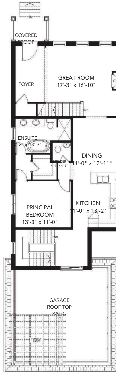
GROUND FLOOR 1397 sq. ft.
