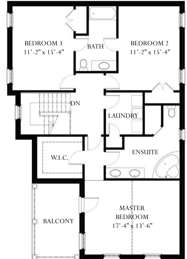
SECOND FLOOR 1217 SQ. FT.
