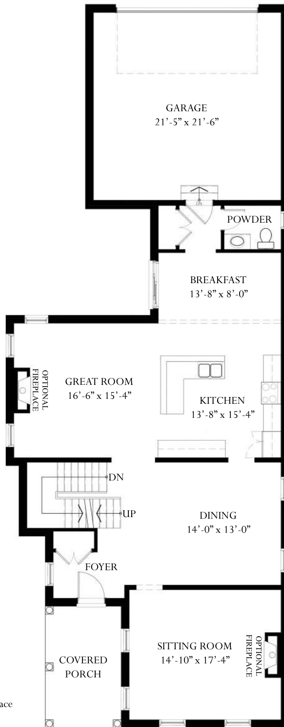
MAIN FLOOR 1423 SQ. FT.
