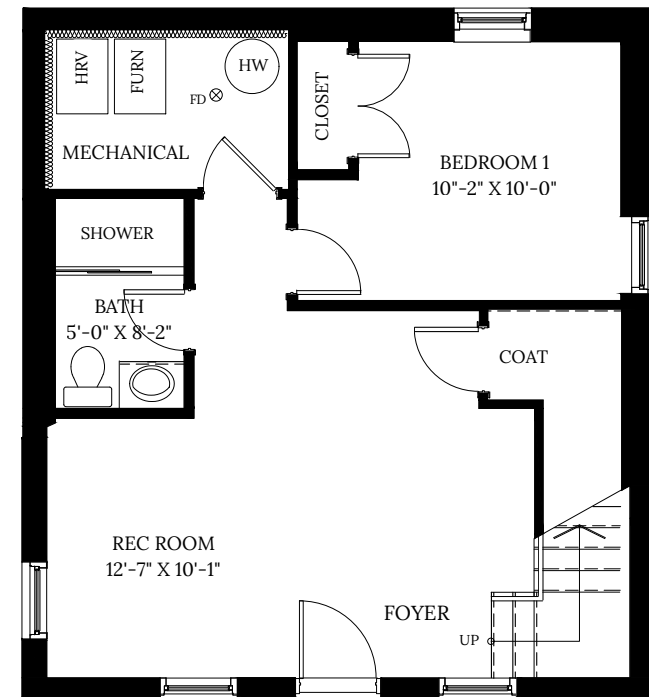
LOWER LEVEL
