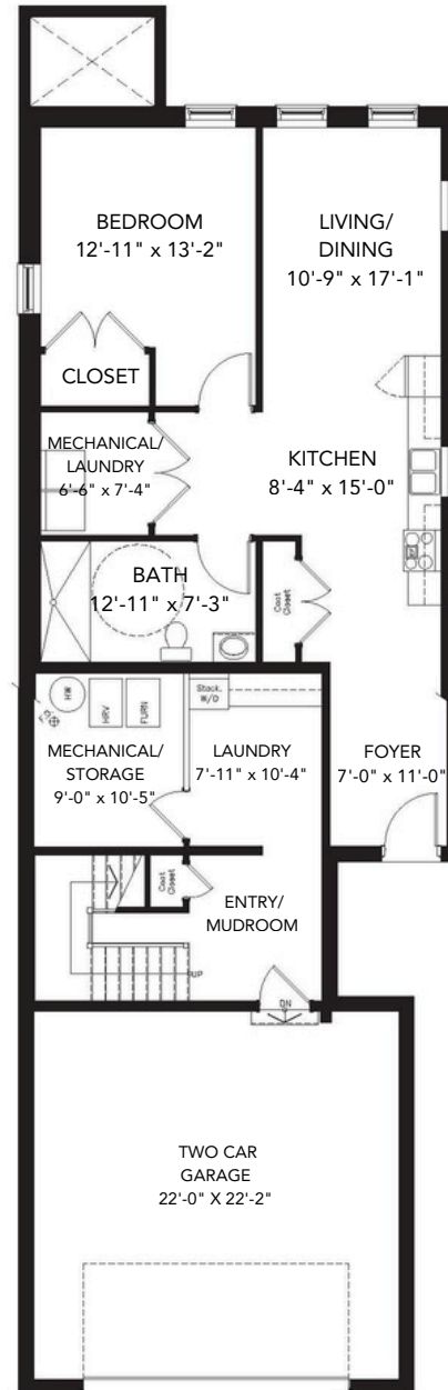
SECONDARY SUITE 988 sq. ft.
