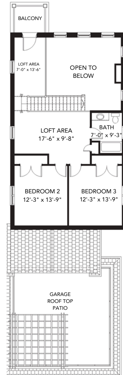
SECOND FLOOR
